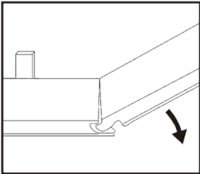
Step 2: Lock short end of plank by inserting tongue into groove at an approximate 30 degrees angle and drop into place. Continue this process throughout the installation.
